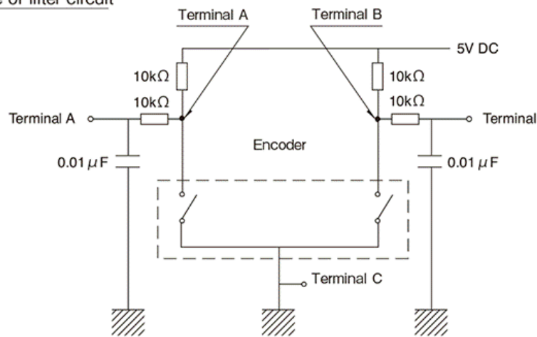
(Example of circuit for use)
